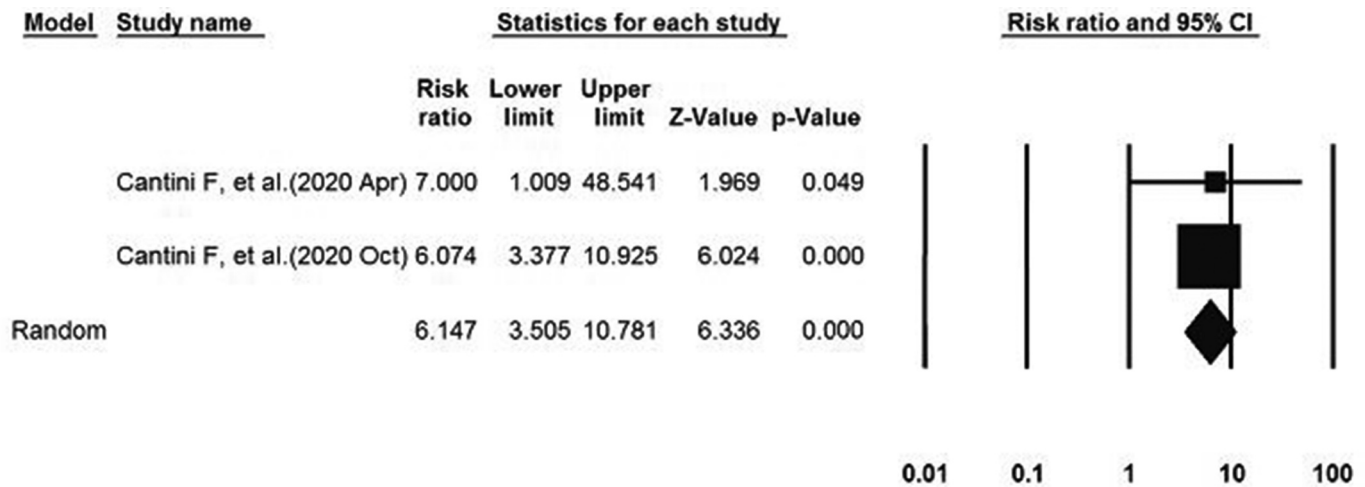
Figure 4. The pooled direct comparison effect of baricitinib therapy versus standard treatment on the discharge rate of the patients with COVID-19 pneumonia related to cohort studies.
