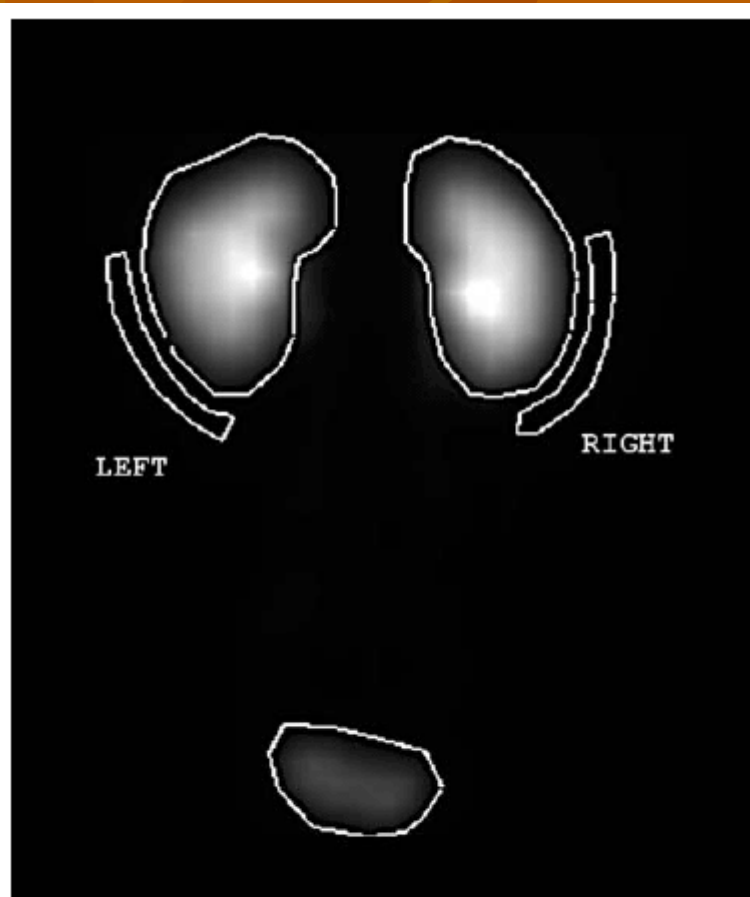
Figure 1 – Regions of interest (ROIs) drew manually in a composite image (1 to 3 minutes after the injection) of the ^{99m}\text{Tc} -DTPA or ^{99m}\text{Tc} -EC dynamic scintigraphies.
