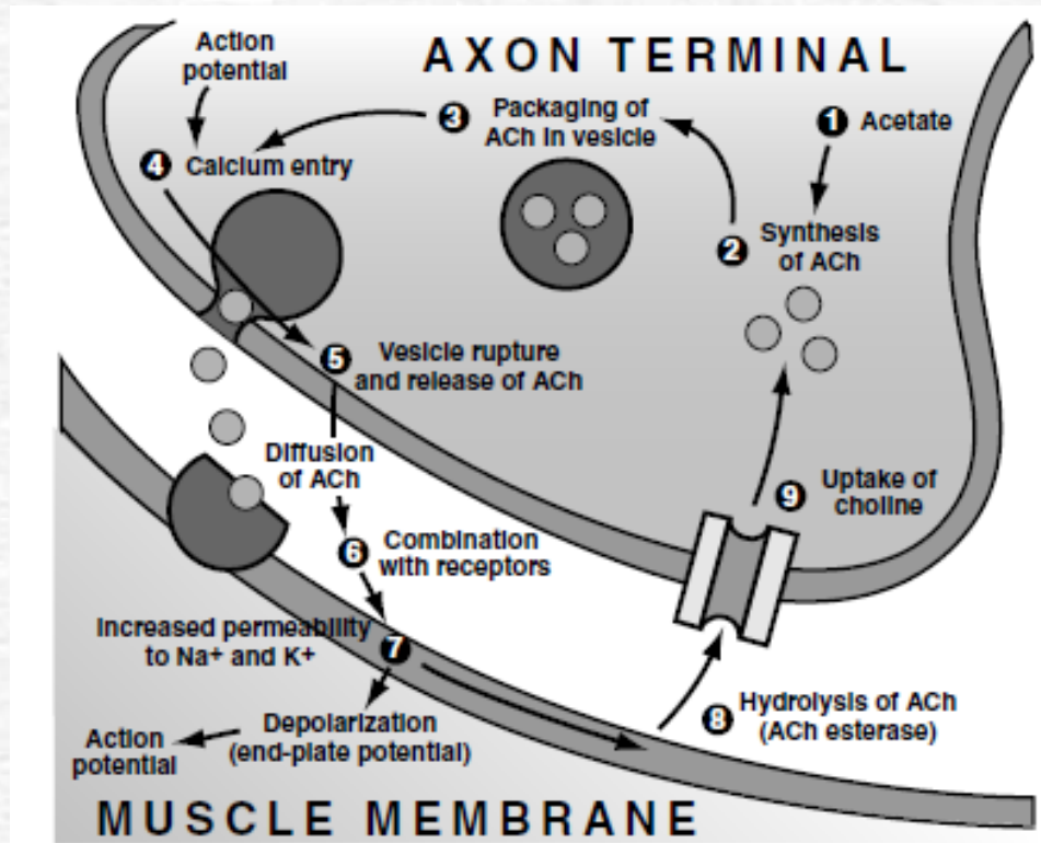
FIGURE 5-10 Acetylcholine release and recycling.
