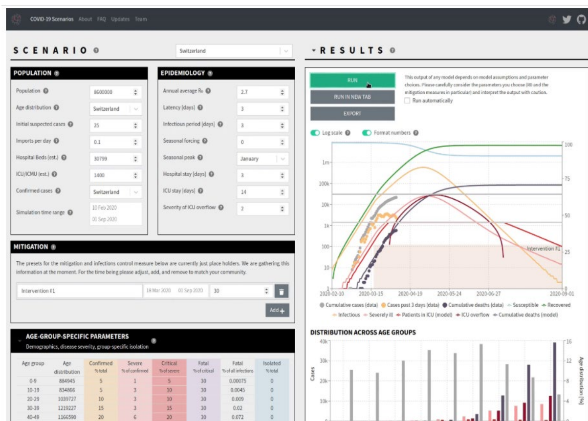
Figure 4. COVID-19 model outbreak trajectories and hospital demand
